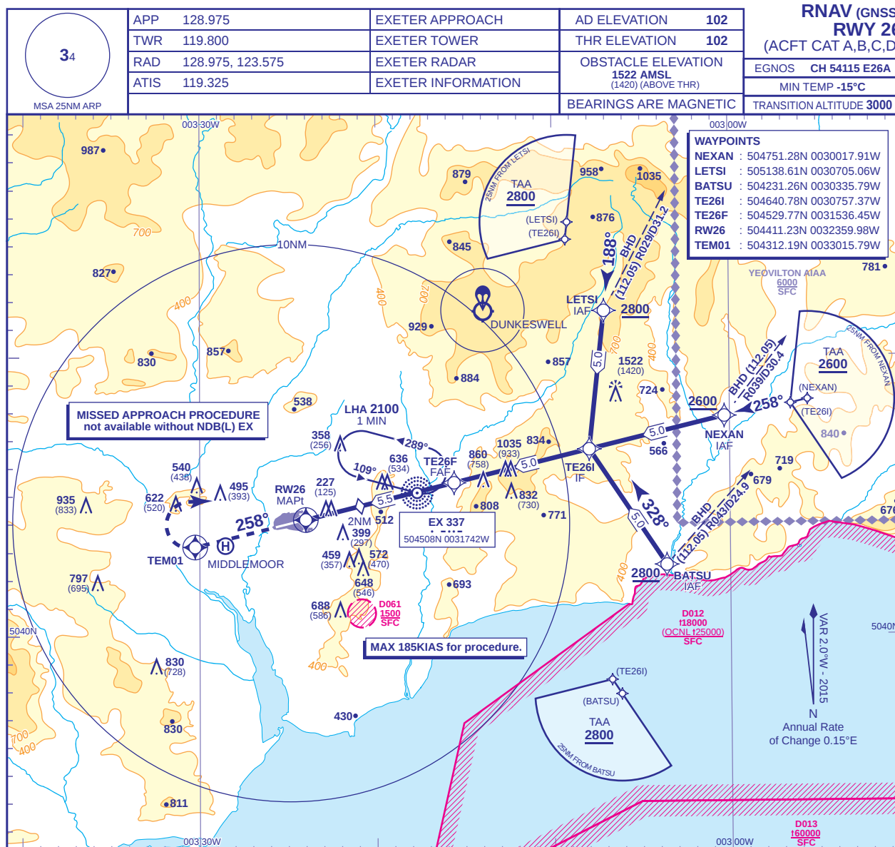
RECOMMENDED PROFILE VNAV - Vertical path Angle 3.5° (LNAV 6.12%), 372FT/NM
