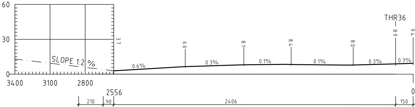
VERTICAL SCALE 1:2000
